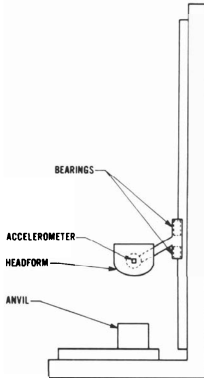
FIGURE 4. Impact attenuation test setup.
