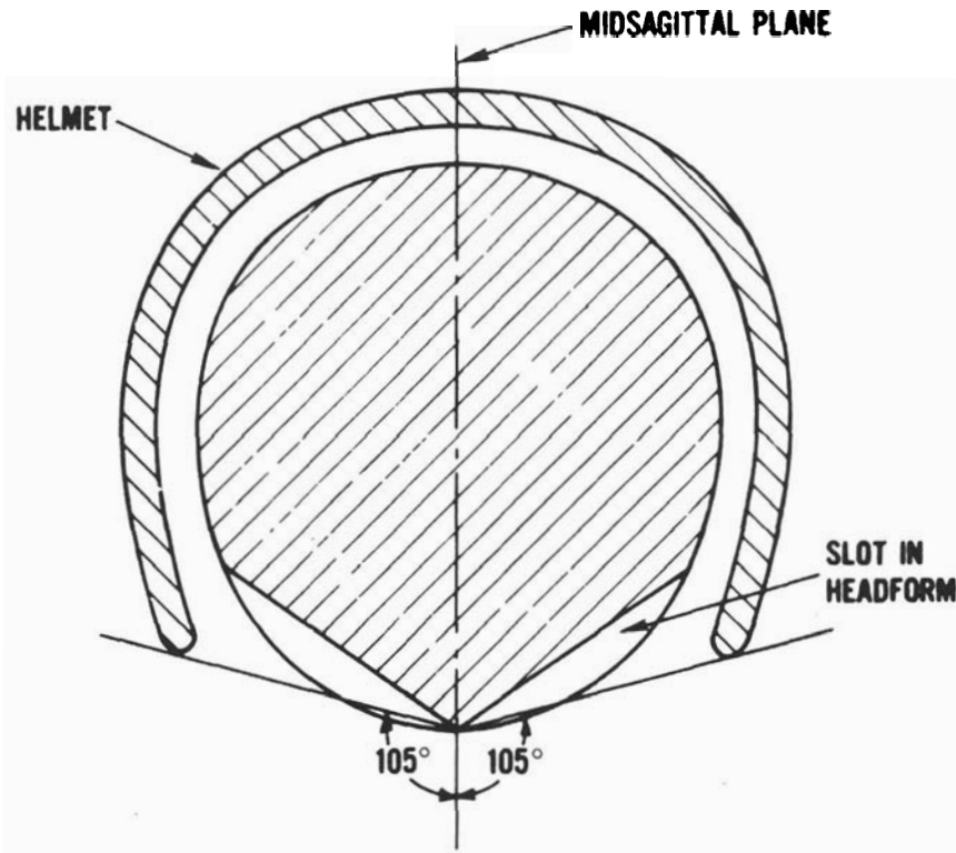
FIGURE 2. Peripheral vision test.
