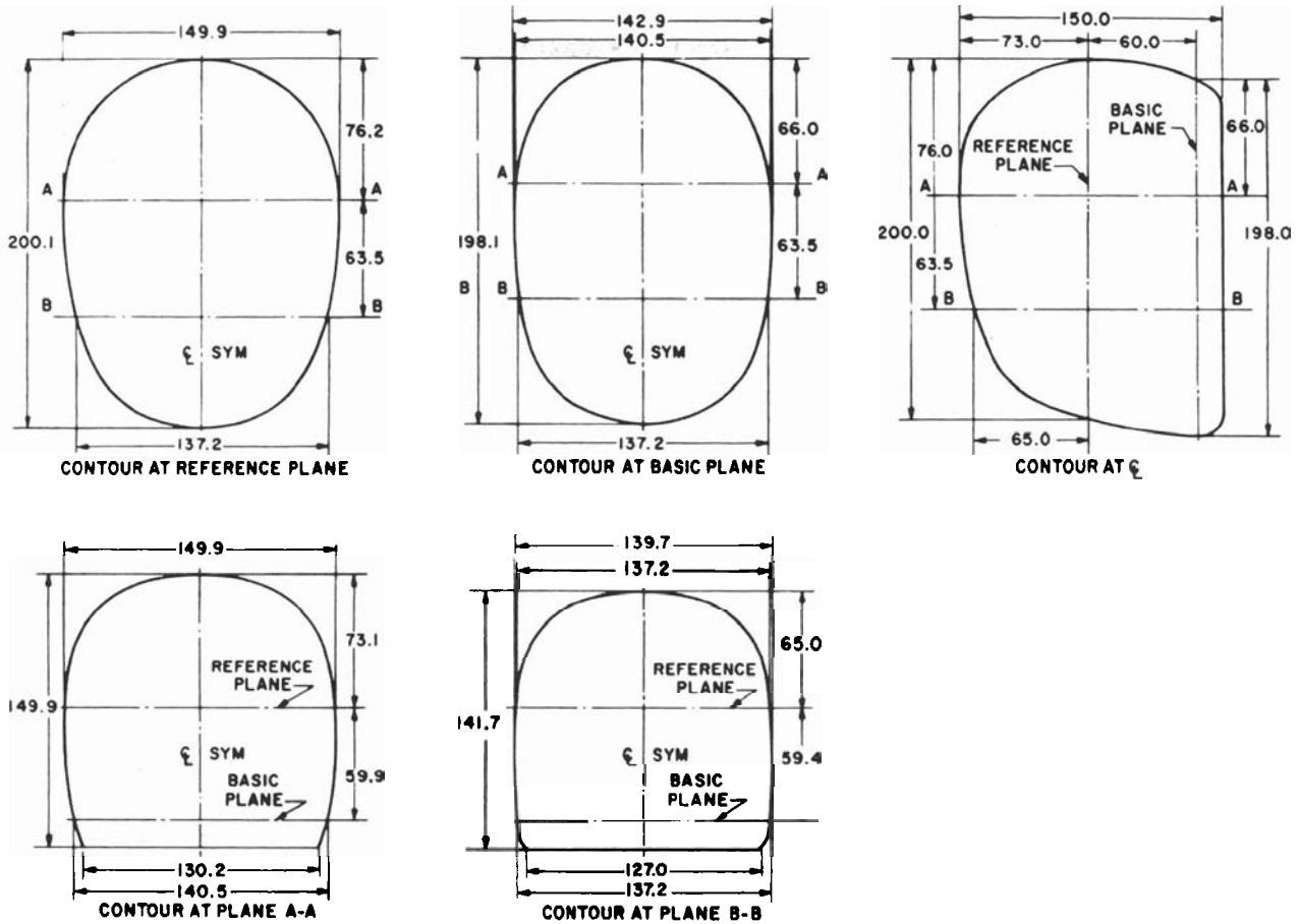
FIGURE 3. Size 7-1/4 test headform, dimensions in millimeters.
